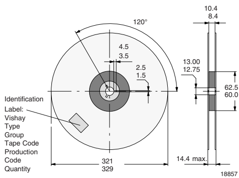
Figure 31. Reel Dimensions - GS18
